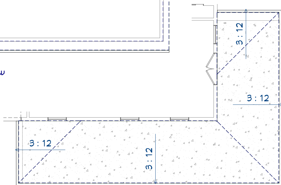
Porch Roof Plan View
