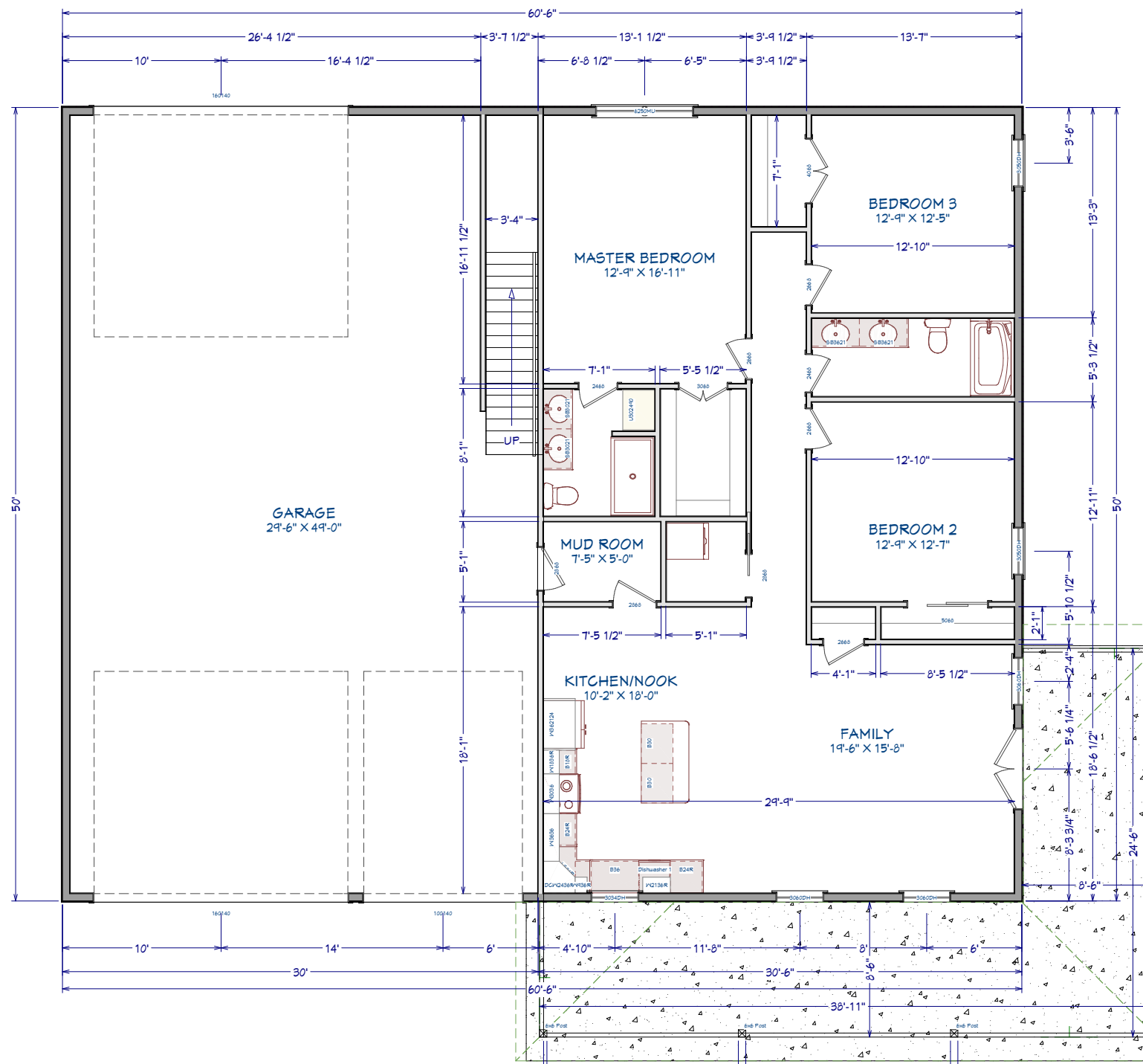
1st Floor
