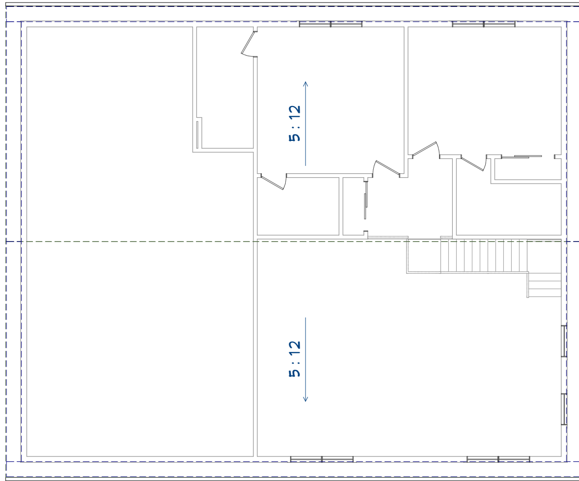
Roof Plan View
