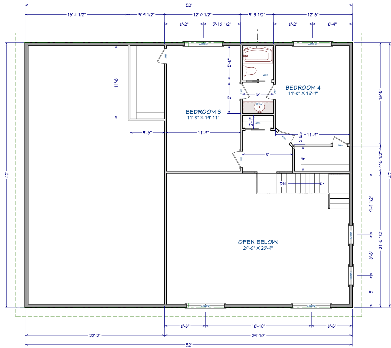
2nd Floor
